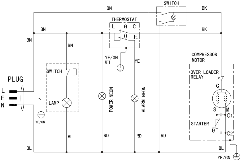
ELECTRIC WIRING DIAGRAM C1 C2: CAPACITOR IS OPTIONAL
