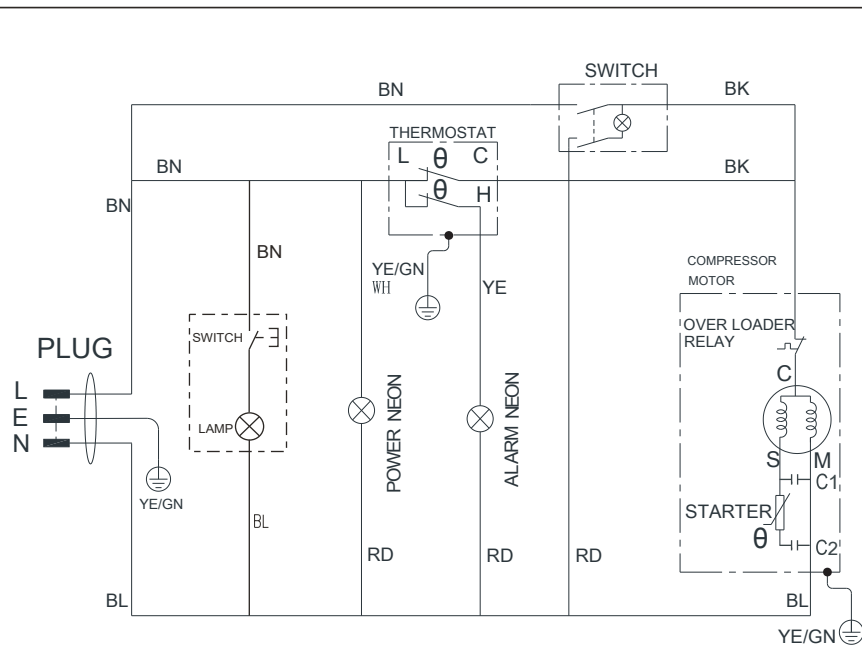
ELECTRIC WIRING DIAGRAM C1 C2: CAPACITOR IS OPTIONAL
