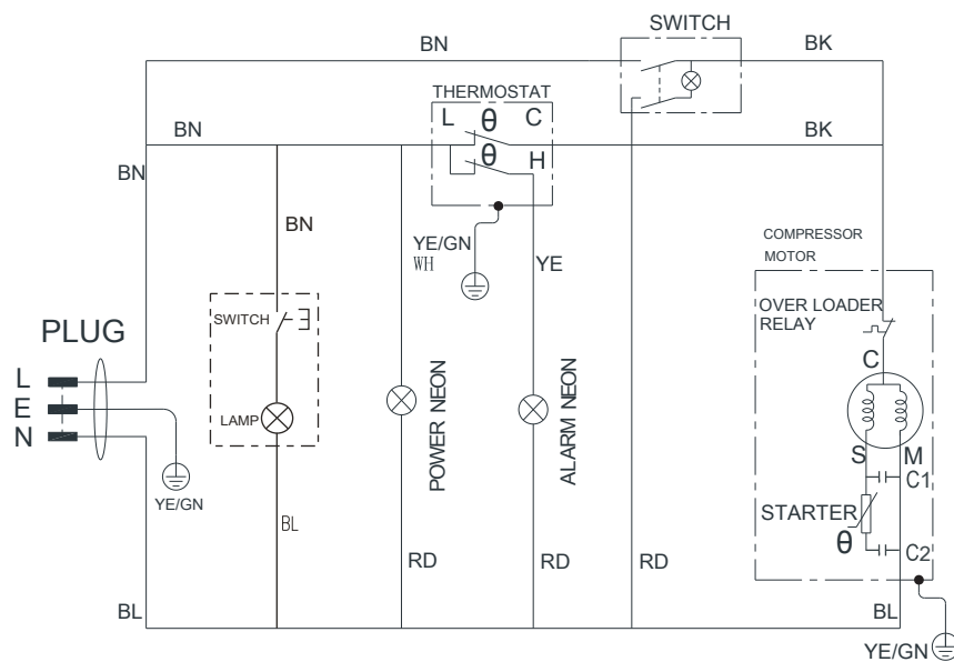
ELECTRIC WIRING DIAGRAM C1 C2: CAPACITOR IS OPTIONAL
