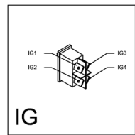
Main switch
