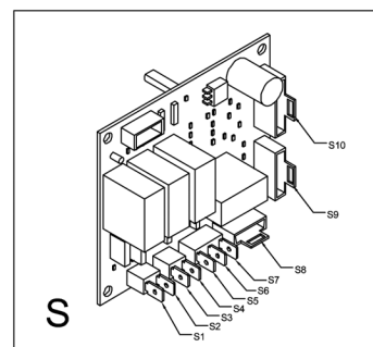
P.c. board
