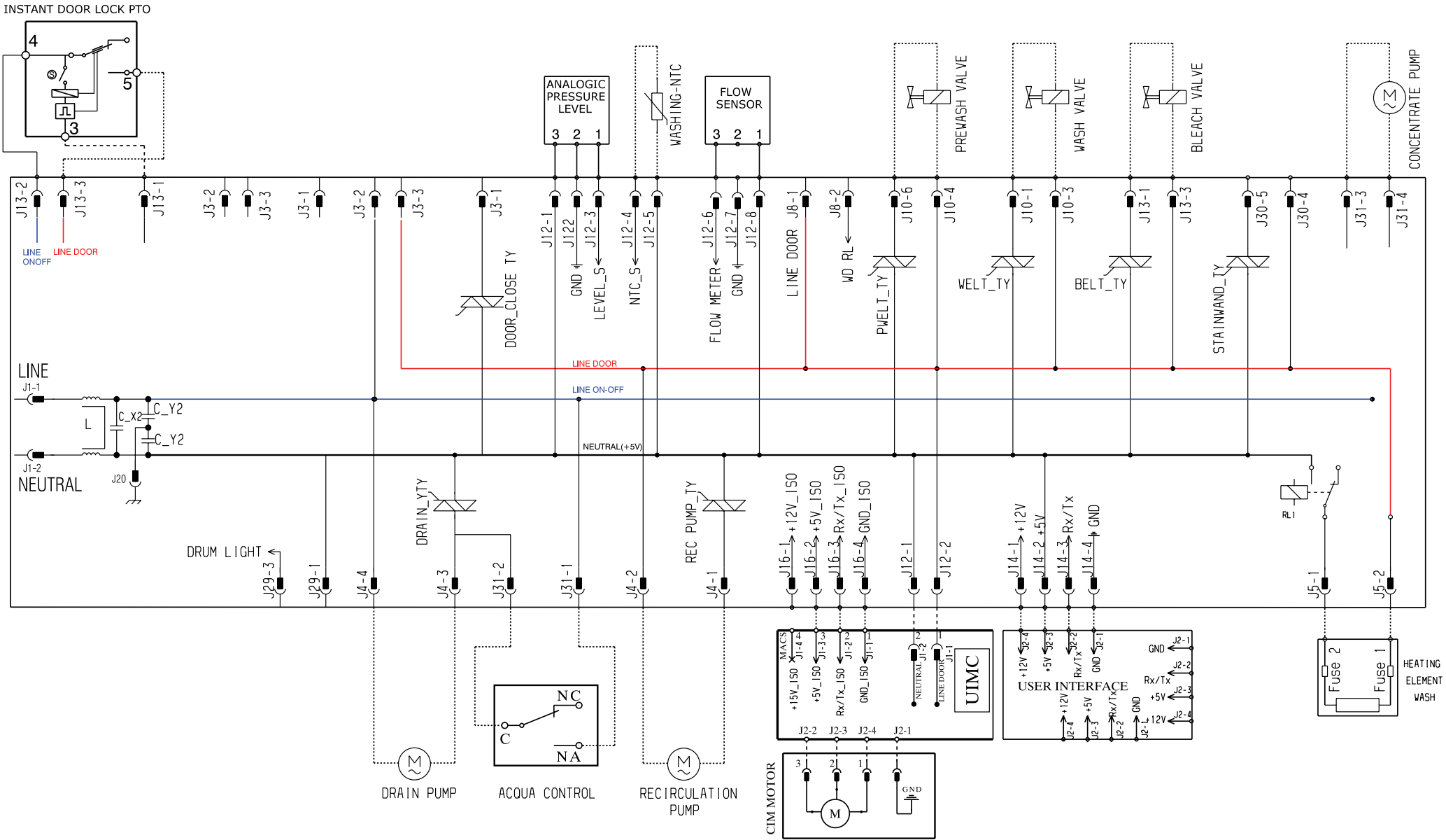
ELECTRIC DIAGRAM EVWX14
