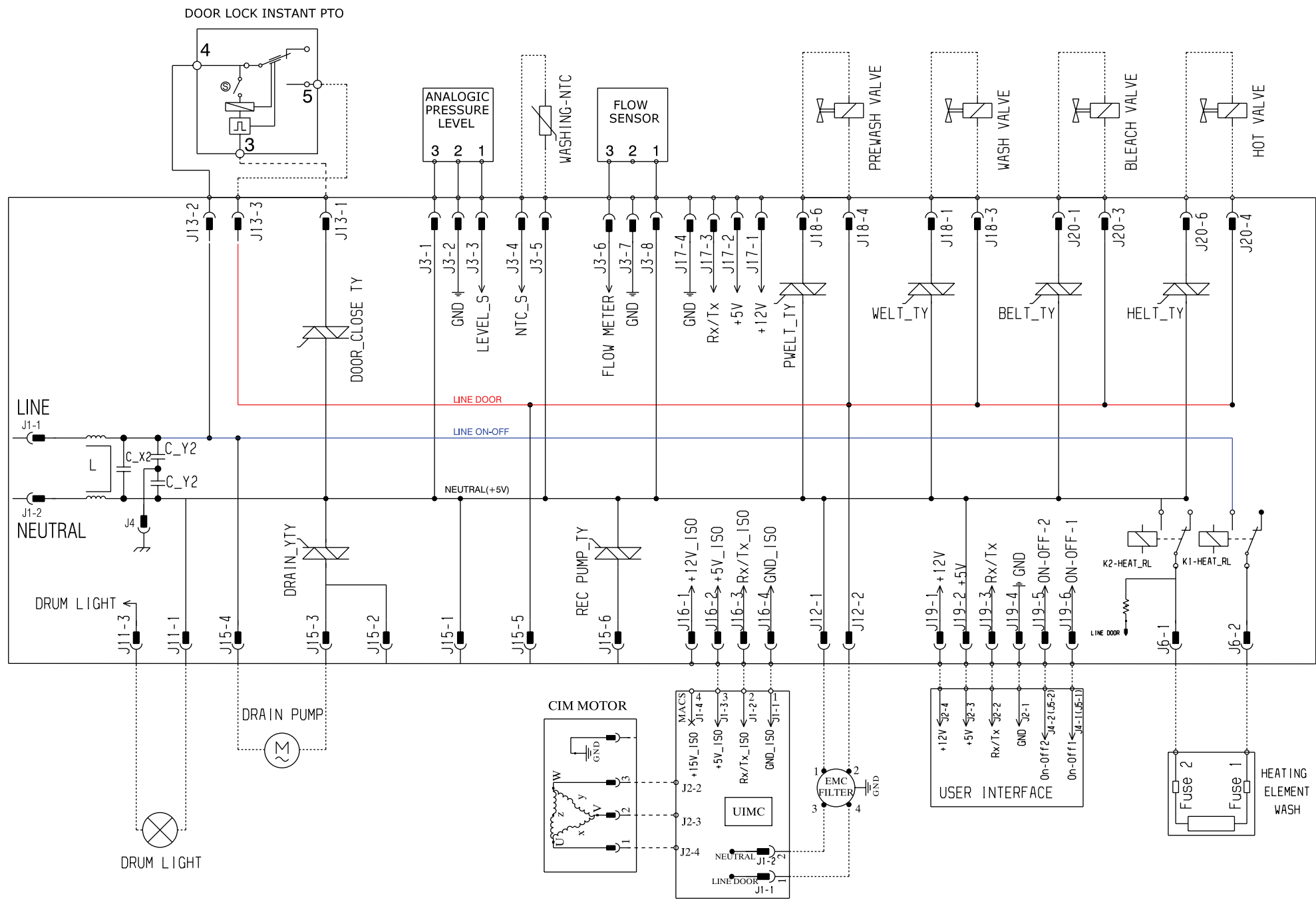
ELECTRIC DIAGRAM EWX11
