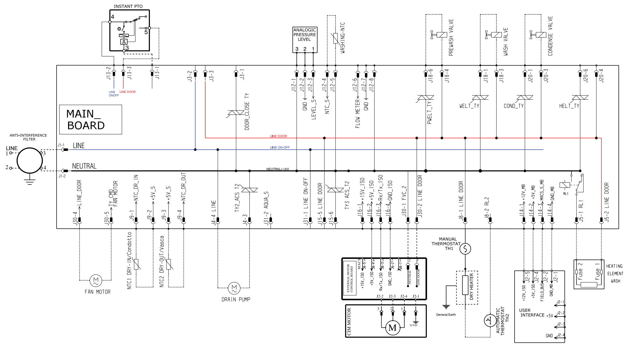
ELECTRIC DIAGRAM EWX14 WD
