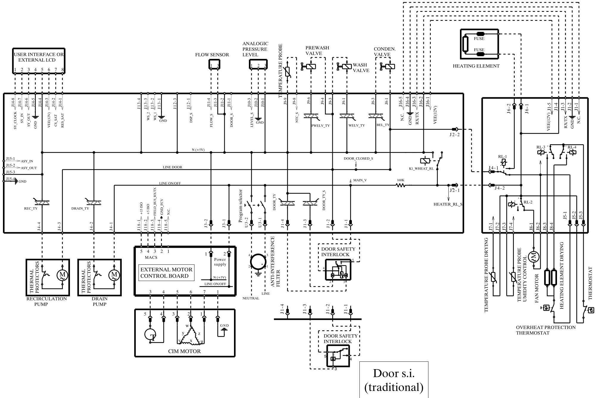
ELECTRIC DIAGRAM
