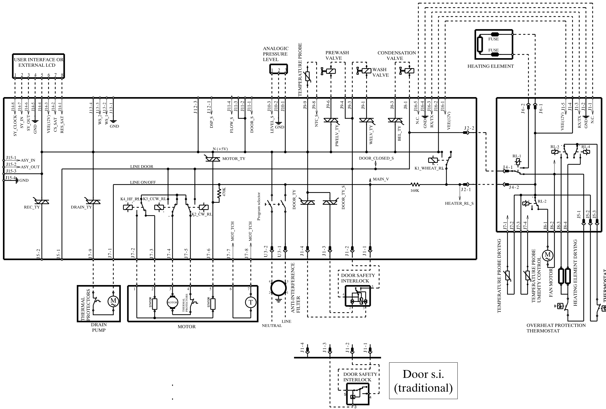
ELECTRIC DIAGRAM
