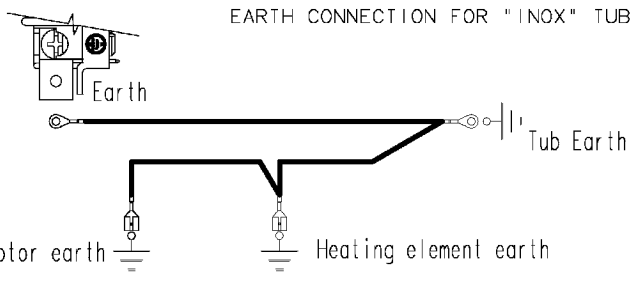
EARTH CONNECTION FOR "INOX" TUB
