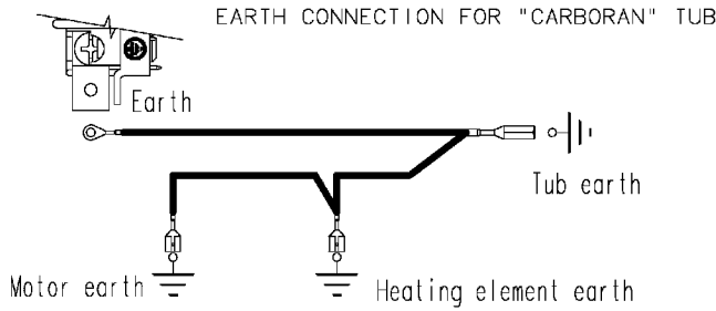
EARTH CONNECTION FOR "CARBORAN" TUB
