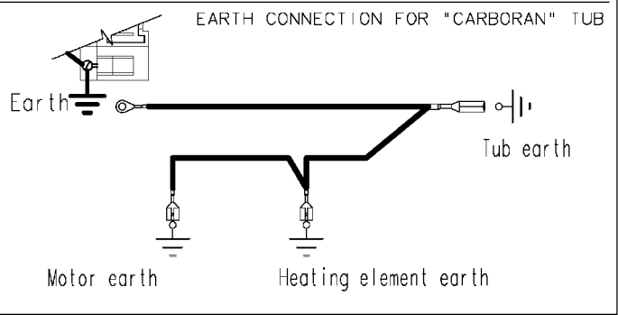
EARTH CONNECTION FOR "CARBORAN" TUB
