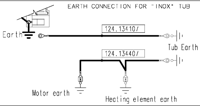
EARTH CONNECTION FOR "INOX" TUB
