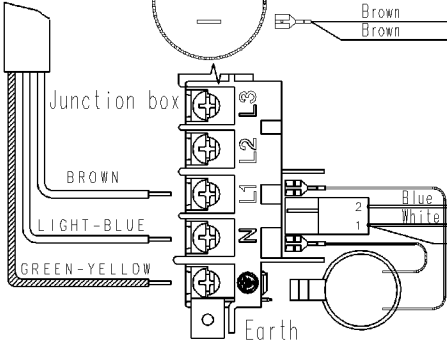
EARTH CONNECTION FOR "INOX" TUB
