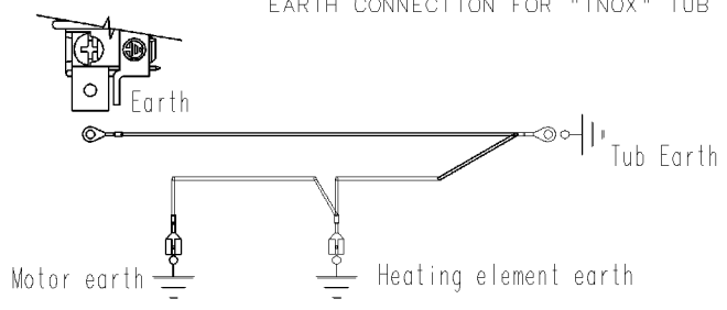
EARTH CONNECTION FOR "INOX" TUB
