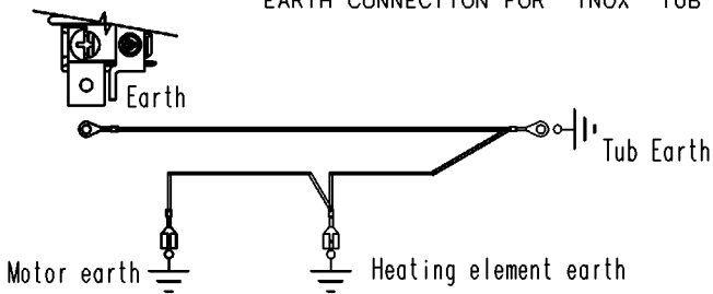
EARTH CONNECTION FOR "INOX" TUB
