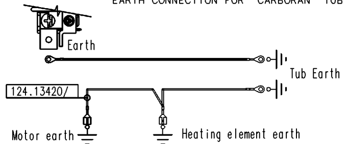
EARTH CONNECTION FOR "CARBORAN" TUB
