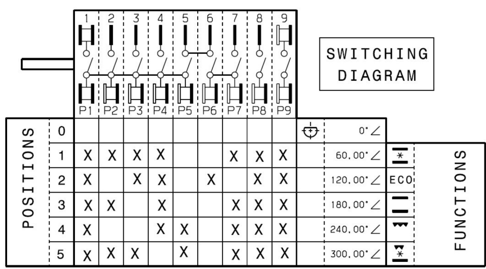
ANC ROTARY SWITCH: A12616301
