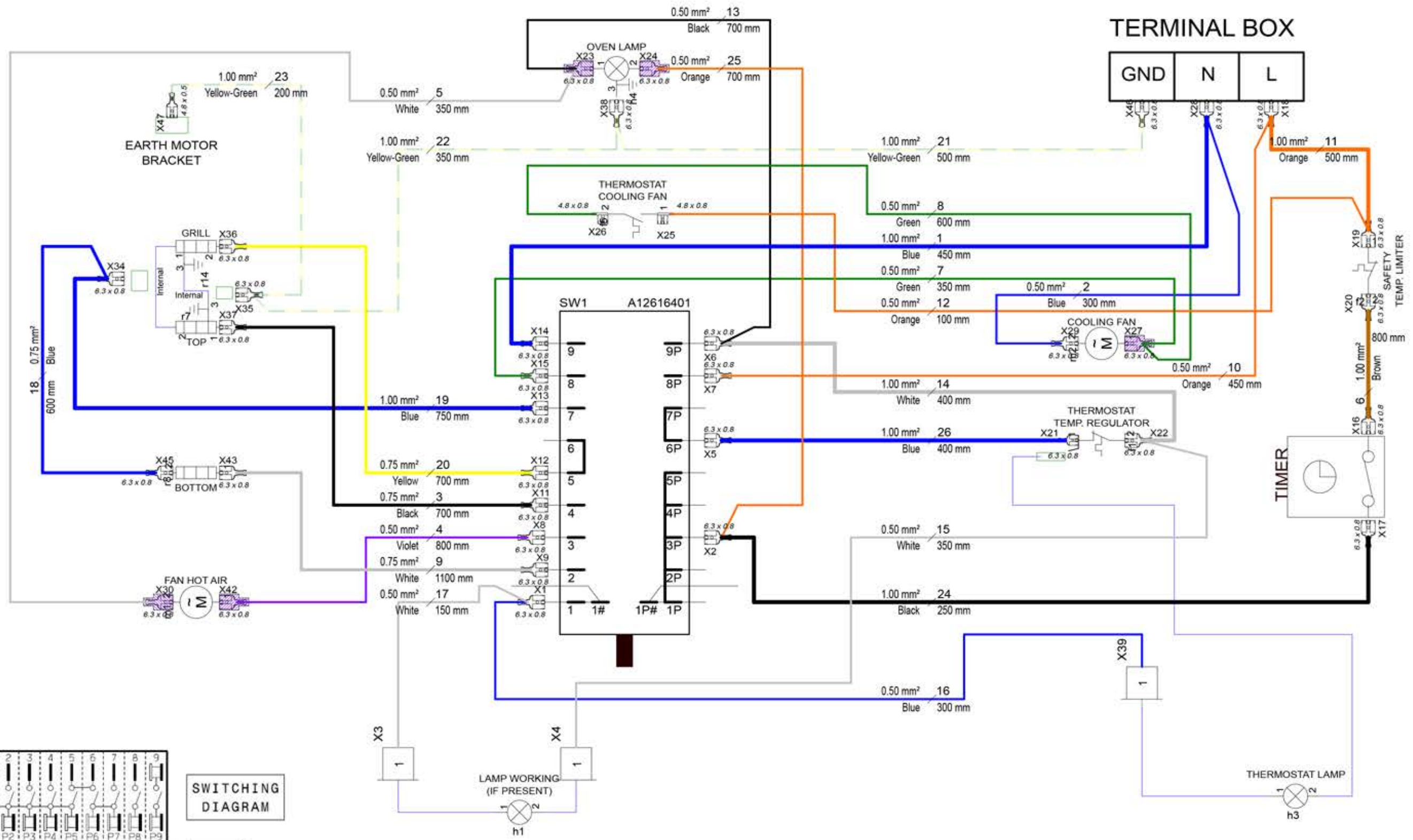
ANC ROTARY SWITCH: A12616401
