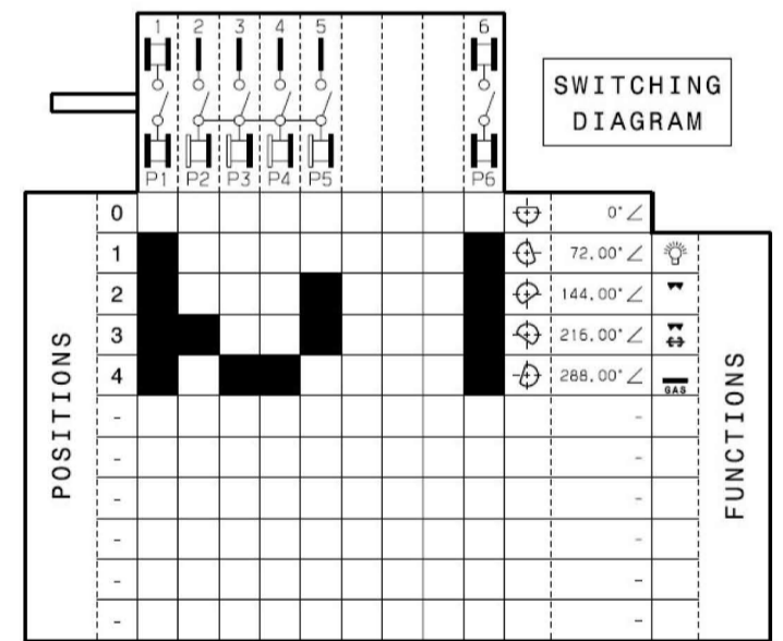
OVEN SWITCH (a7) 807179401
