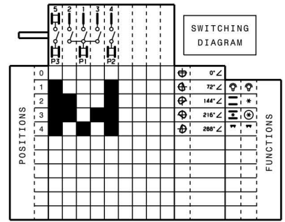
OVEN SWITCH 807179402
