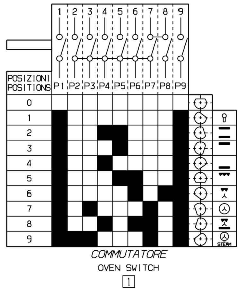
ELECTRIC DIAGRAM DIAGRAMMA ELETTRICO
