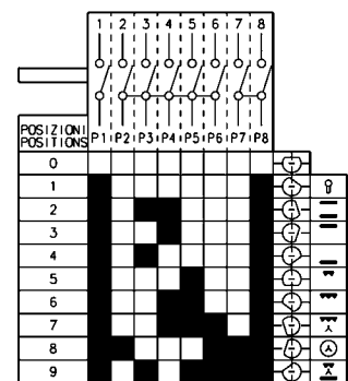
OVEN SWITCH 1
