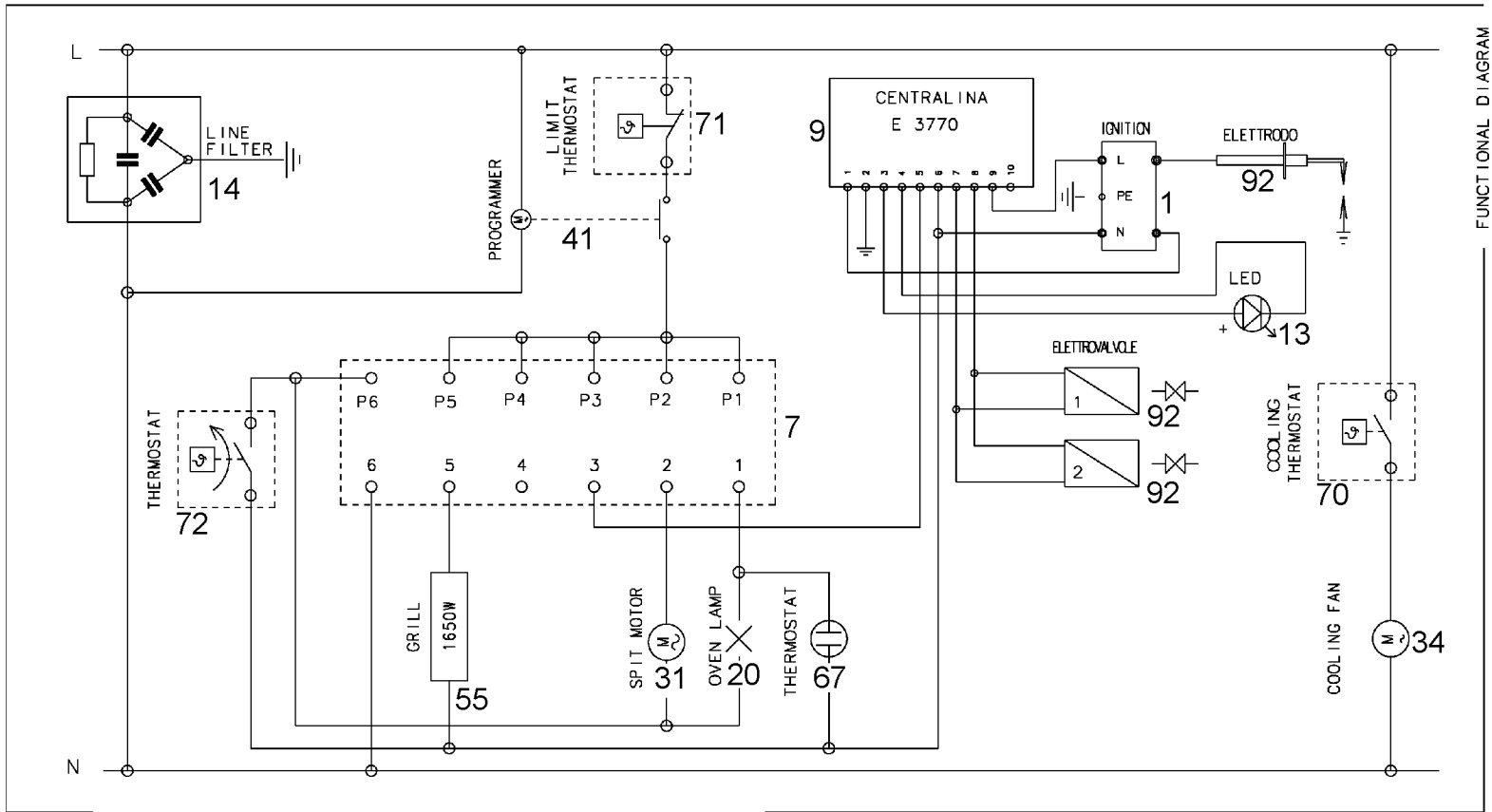
ELECTRIC DIAGRAM DIAGRAMMA ELETTRICO
