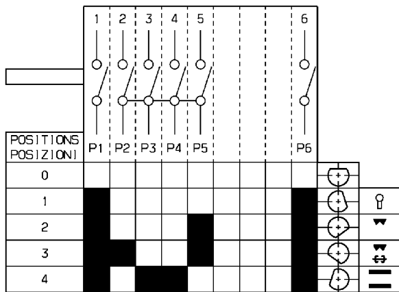
OVEN SWITCH [1]
