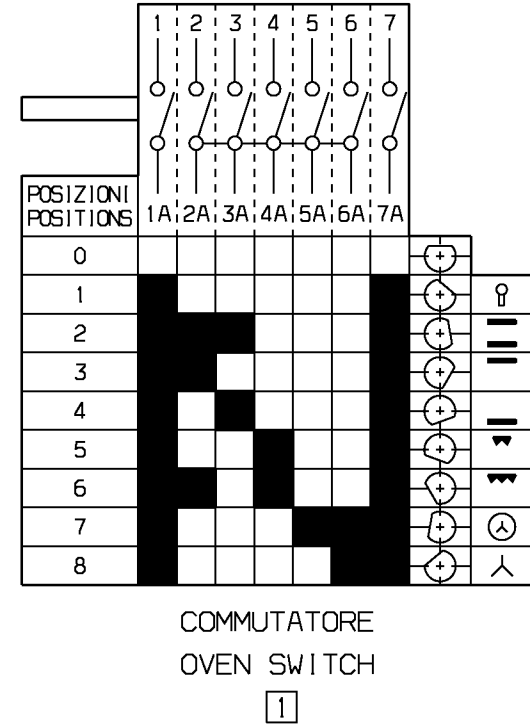
ELECTRIC DIAGRAM DIAGRAMMA ELETTRICO
