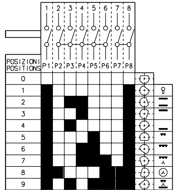
OVEN SWITCH 1
