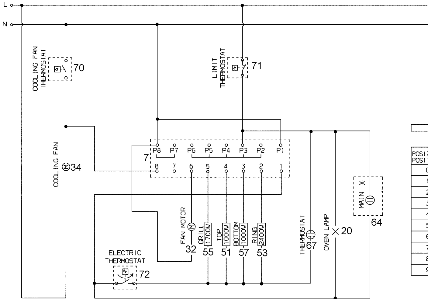
ELECTRIC DIAGRAM DIAGRAMMA ELETTRICO
