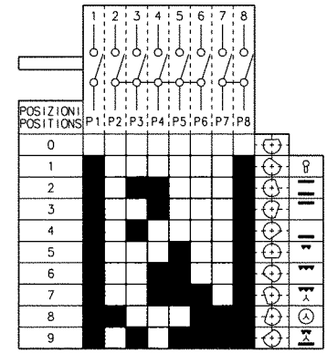
OVEN SWITCH 1
