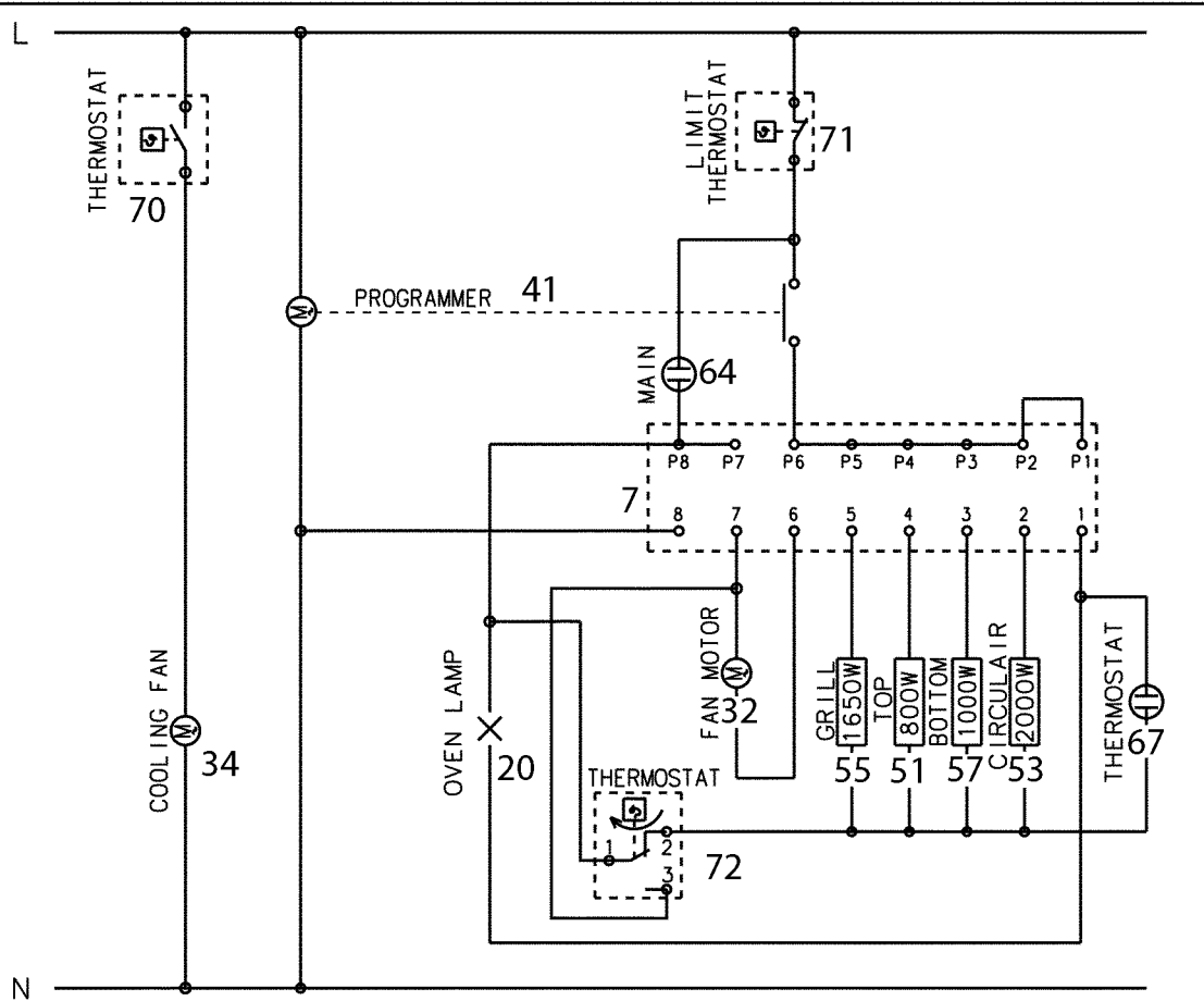
ELECTRIC DIAGRAM
