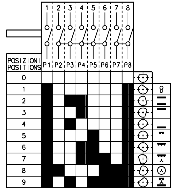
OVEN SWITCH 1
