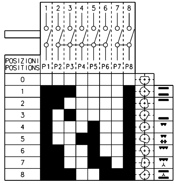
OVEN SWITCH 1
