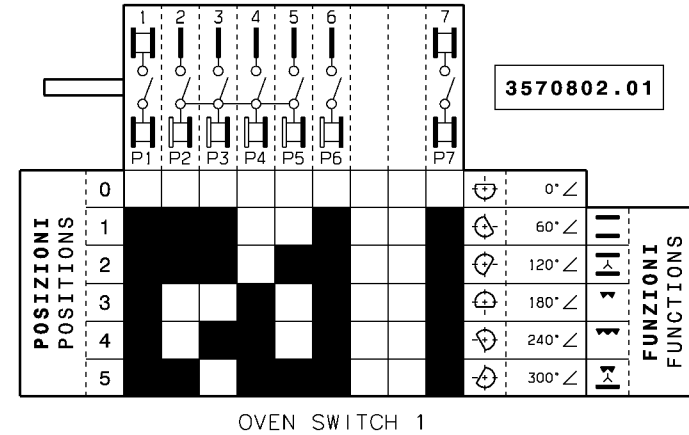
ELECTRIC DIAGRAM DIAGRAMMA ELETTRICO
