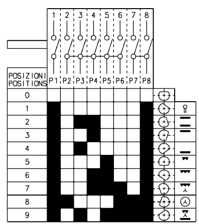
OVEN SWITCH 1
