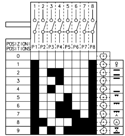
OVEN SWITCH 1
