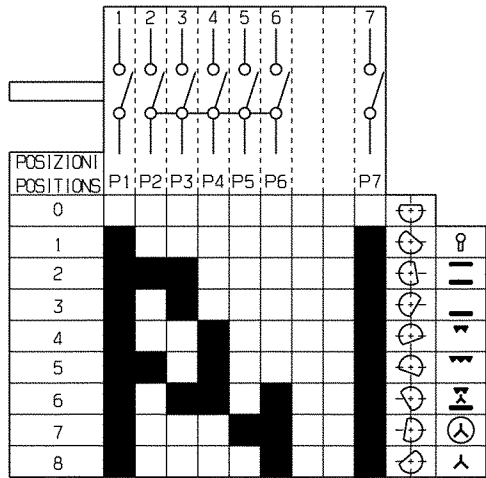
DIAGRAMMA ELETTRICO ELECTRIC DIAGRAM
