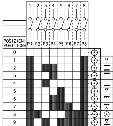
OVEN SWITCH 1
