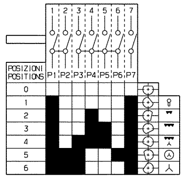
OVEN SWITCH 1
