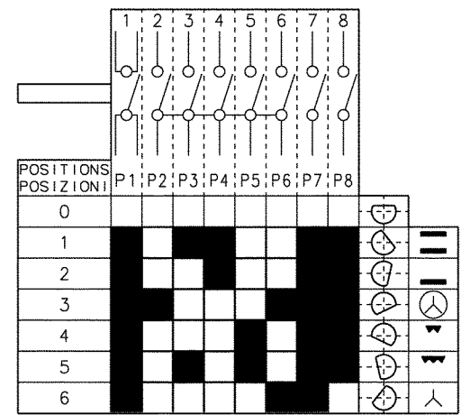
OVEN SWITCH 1
