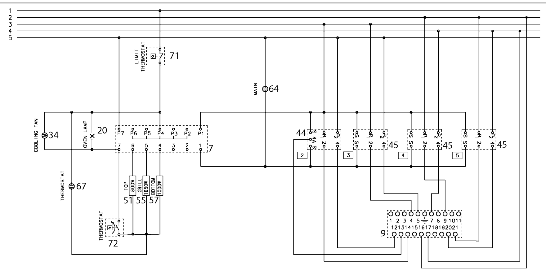
ELECTRIC DIAGRAM
