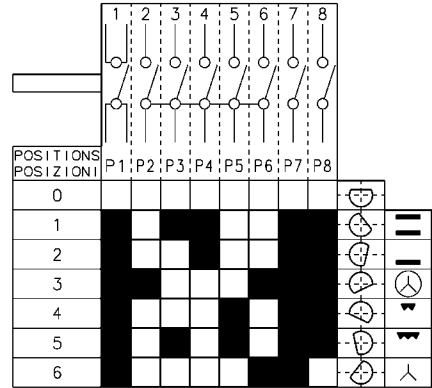
OVEN SWITCH 1
