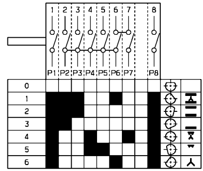
OVEN SWITCH
