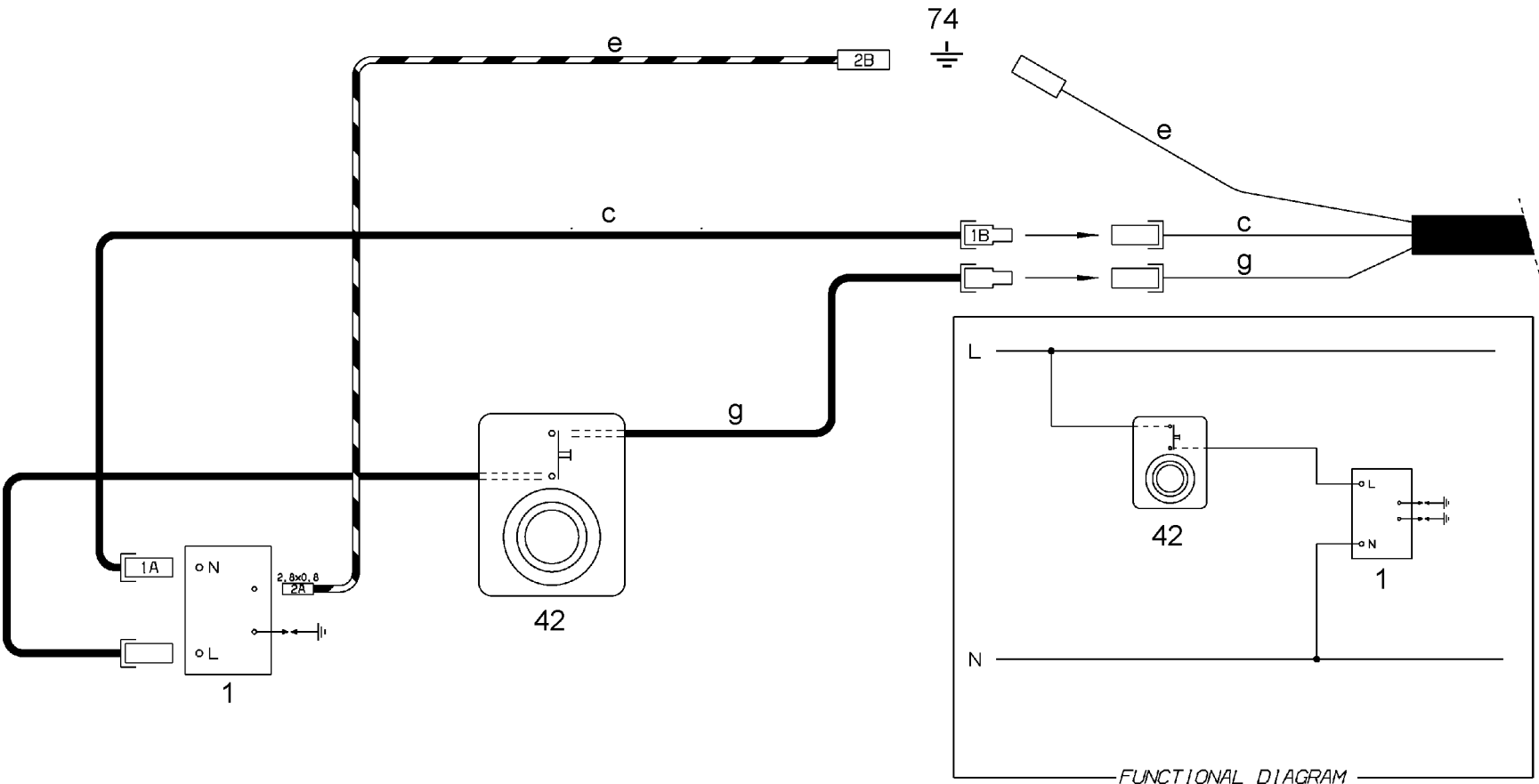
FUNCTIONAL DIAGRAM
