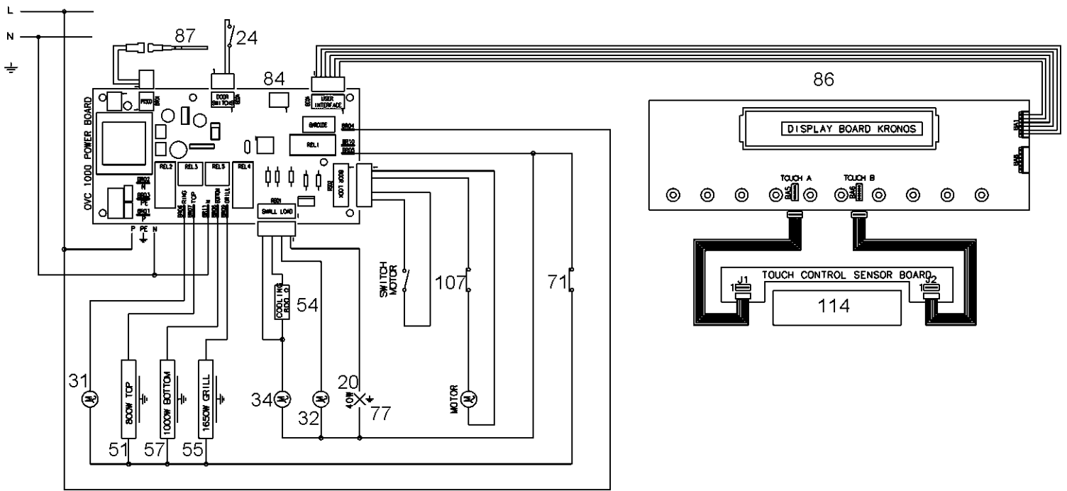
FUNCTIONAL DIAGRAM
