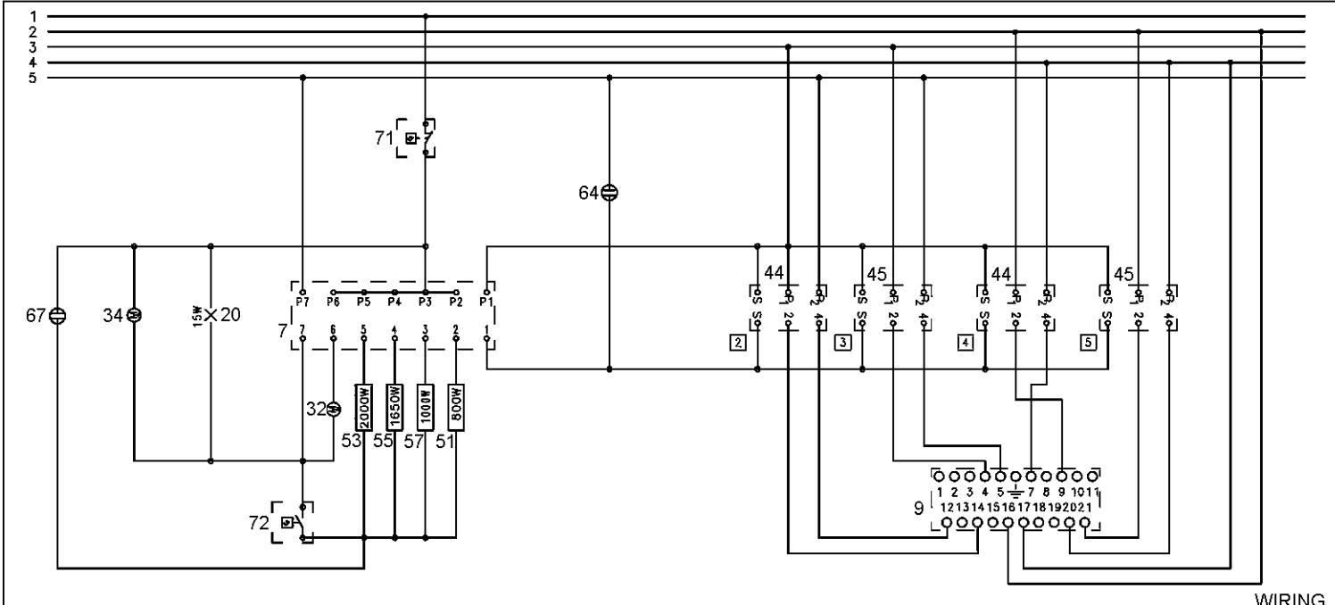
SINGLE ENERGY REGULATOR [2|3|4|5]
