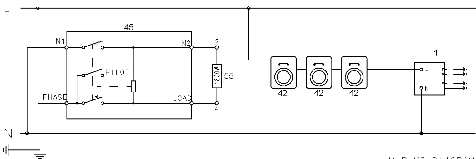
WIRING DIAGRAM
