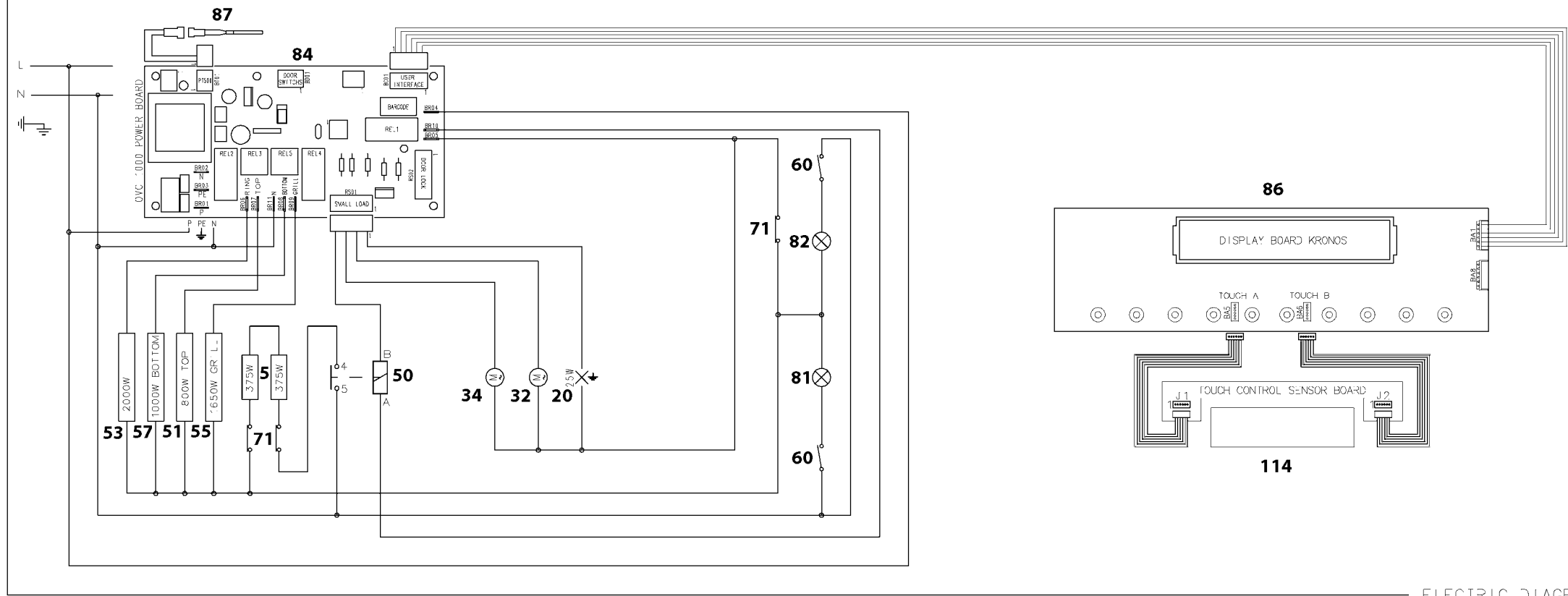
ELECTRIC DIAGRAM
