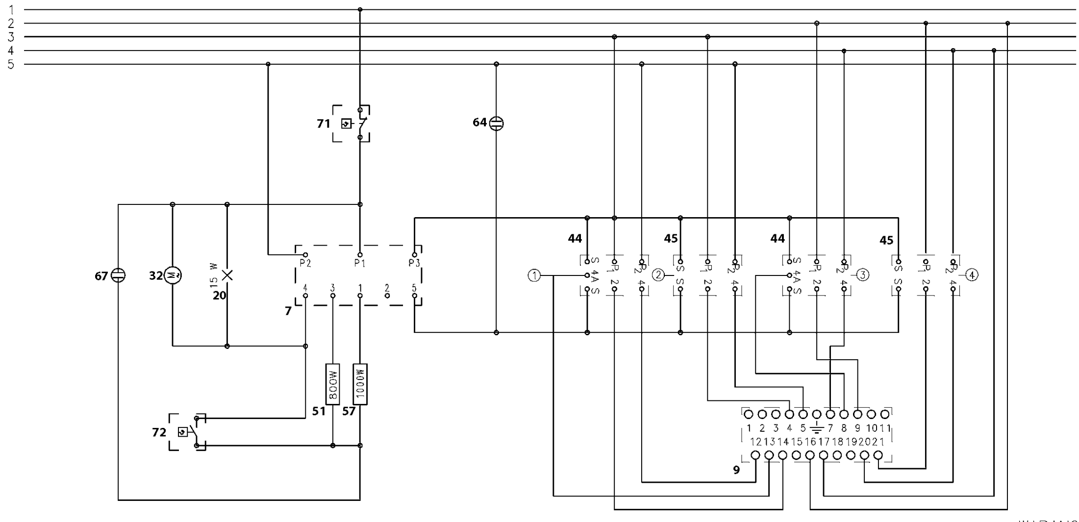
SINGLE ENERGY REGULATOR [2|4]
