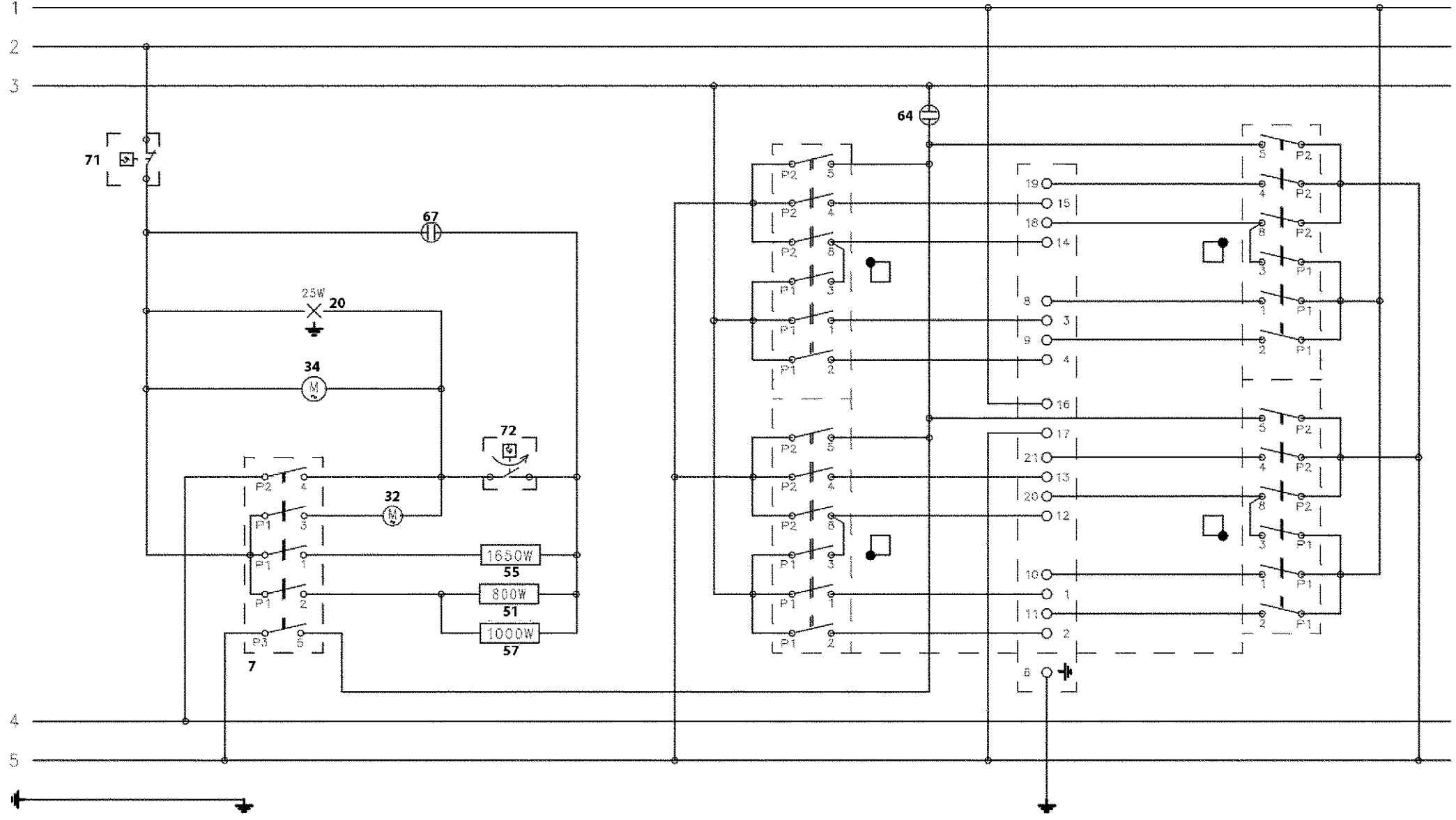
FUNCTIONAL DIAGRAM
