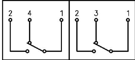
OVEN SWITCH 1
