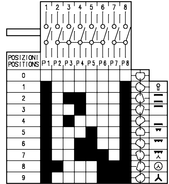
OVEN SWITCH 1
