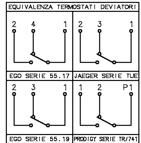
OVEN SWITCH 1
