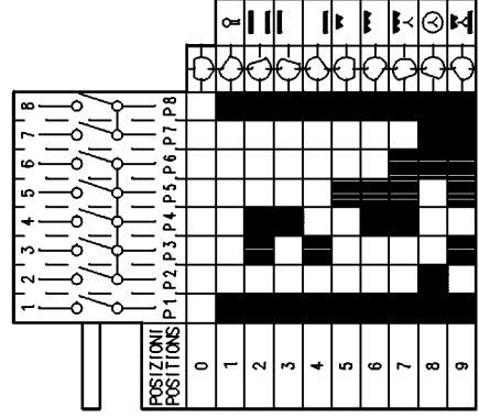
OVEN SWITCH 1
