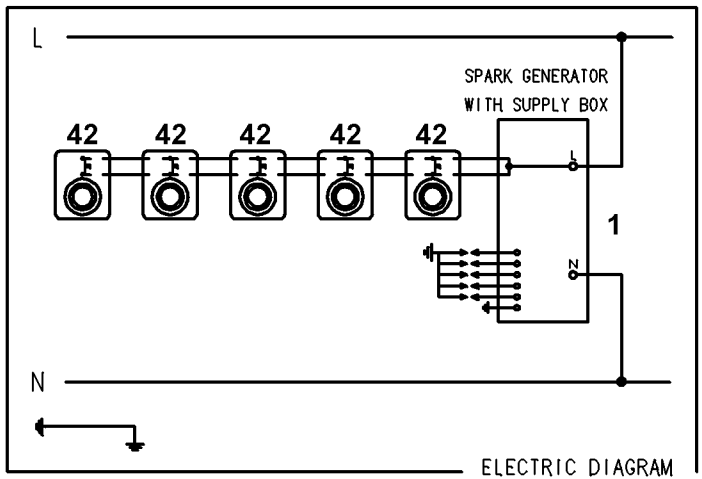
ELECTRIC DIAGRAM
