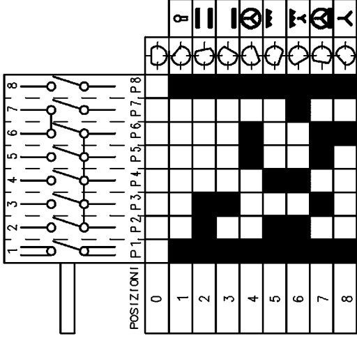
OVEN SWITCH ①
