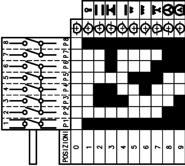
MULTIFUNCTION OVEN SWITCH ①
